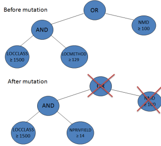
Fig 5. Mutation operator
